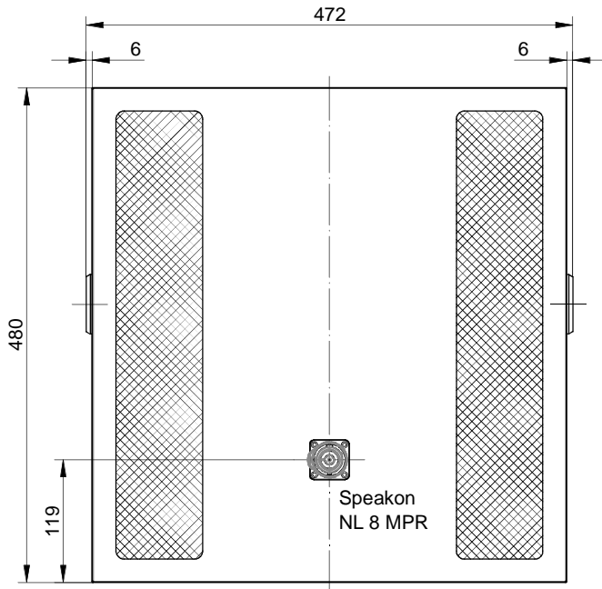
Rear view
