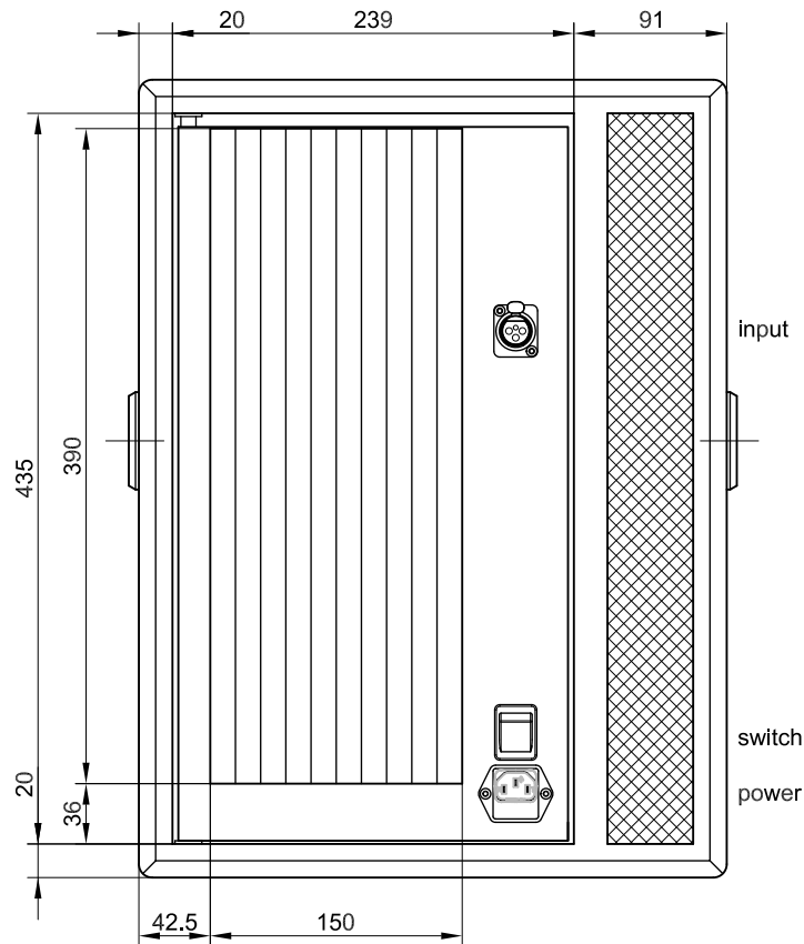
Rear view
