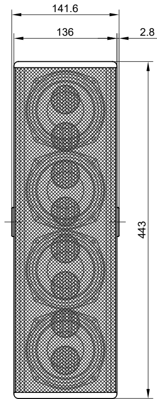
Front view
