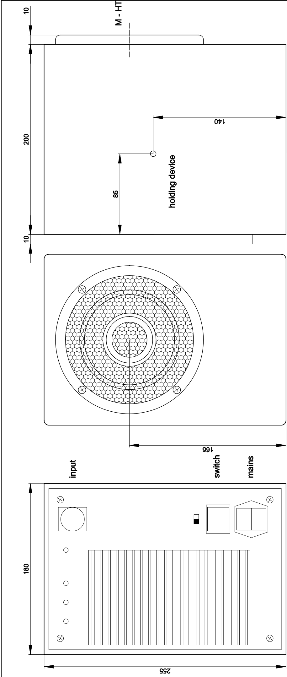
Side view
