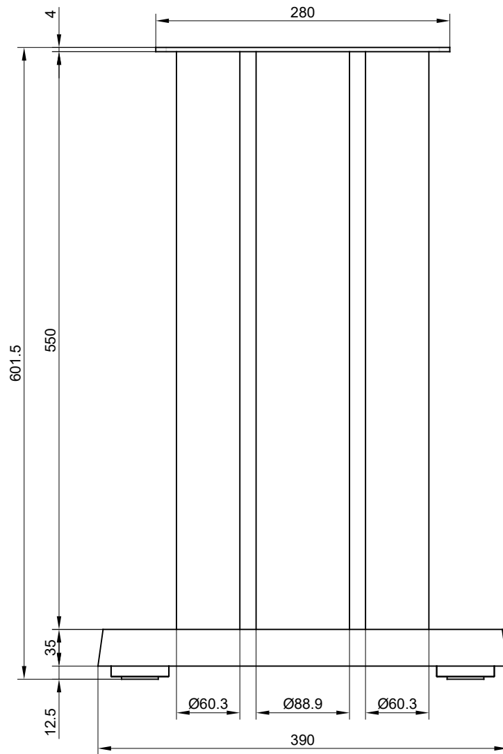
Front view
