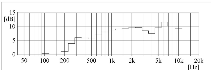
Directivity index
