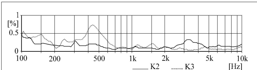
Total harmonic distortion P_A = 90 dB
